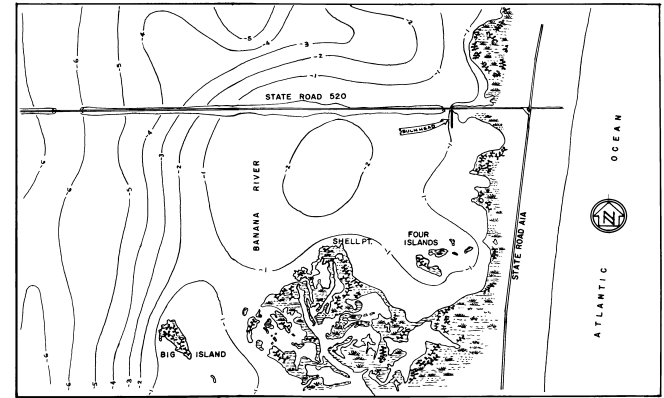
LOCATION PLAN TAKEN FROM UNITED STATES GEOLOGICAL SURVEY QUADRANGLE SHEET N° N 2815. SCALE 1" = 2000' 2000 1000 0 1000 2000
